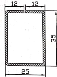
ST25×35 UP86 UP86-M
