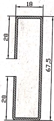
ST18×67.5 UP72-96 UP72-96-N
